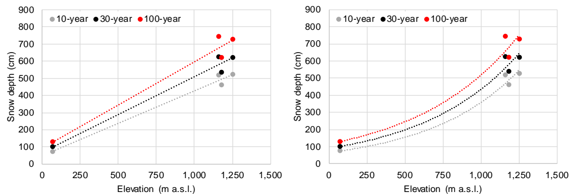
Figure 4. Predicted snow depths for snow course stations near Hemlock Valley, using a linear approach (left) and exponential approach (right).
