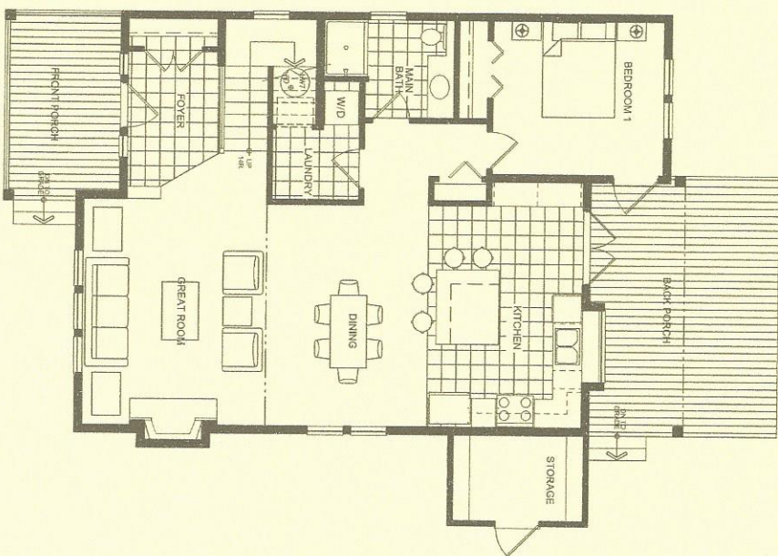
Main Floor Main Area: 1062 sq.ft. Total Area: 1578 sq.ft.
