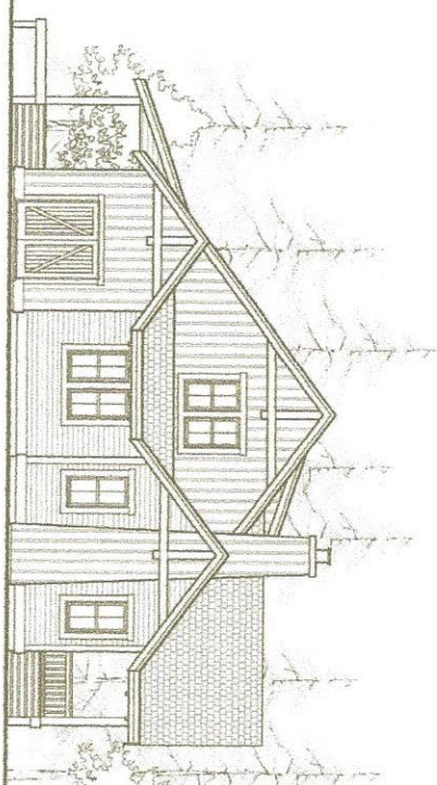
Left Elevation
